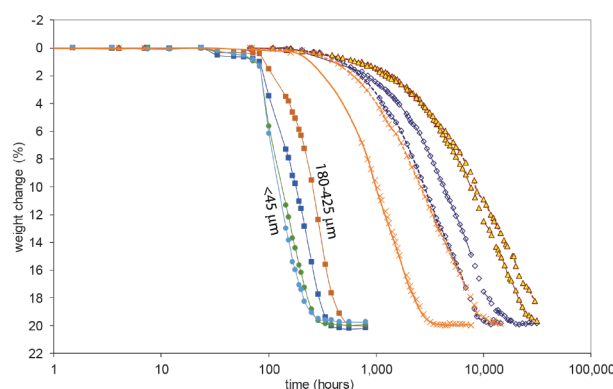
FIGURE 6. Dehydration rates for transformation of gypsum to bassanite at 24 °C and ~0.7 Pa P_{H_2O} . Rates for powdered (<45 µm) to granular (180–425 µm) samples are after Vaniman and Chipera (2006; intermediate curves are for 45–75 and 75–180 µm). Longer dehydration rates are for solid centimeter-scale (2 to 3 g) samples of satin spar (Wildhorse Mesa, Utah = crosses), single selenite crystals (Bingham, New Mexico = diamonds), and nodular evaporite (Todilto formation, New Mexico = triangles). The larger solid samples were run as duplicates and variation in duplicate rates represents variation between sample splits.
